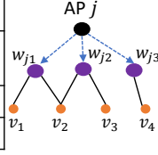
Fig. 2. Example of edge creation for AP j when n_j > 1 : Given that \sum \tilde{x}_{ijm} = 2.4 , we create three AP nodes for AP j (where i denotes the task node index and m indicates the bandwidth allocation level B_m ). The values of \tilde{x}_{ijm} are sorted in descending order of m , and we denote the s -th element in the sorted list as \tilde{x}_{j,s} . Edges between task nodes and AP nodes are then constructed based on this sorted list, with AP nodes ordered as w_{j1}, w_{j2}, w_{j3} . The first element, \tilde{x}_{j,1} , corresponds to \tilde{x}_{1j8} . Therefore, we create an edge (v_1, w_{j1}) between task node v_1 and AP node w_{j1} , with bandwidth allocation b(v_1, w_{j1}) = B_8 and edge fraction F_{\tilde{x}}(v_1, w_{j1}) = \tilde{x}_{1j8} = 0.5 . The second element, \tilde{x}_{j,2} , corresponds to \tilde{x}_{2j7} . Since \tilde{x}_{1j8} + \tilde{x}_{j,2} > 1 , define two edges based on \tilde{x}_{j,2} , (v_2, w_{j1}) and (v_2, w_{j2}) . Specifically, we ensure that the total fraction assigned to each AP node does not exceed 1. For example, F_{\tilde{x}}(v_1, w_{j1}) + F_{\tilde{x}}(v_2, w_{j1}) = 1 , and the remaining portion is assigned as F_{\tilde{x}}(v_2, w_{j2}) = \tilde{x}_{1j8} + \tilde{x}_{j,2} - 1 = 0.5 . The edge construction process continues similarly for the remaining elements \tilde{x}_{j,s} in the sorted list.
